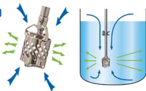
Rotosolver® High Shear Mixer
